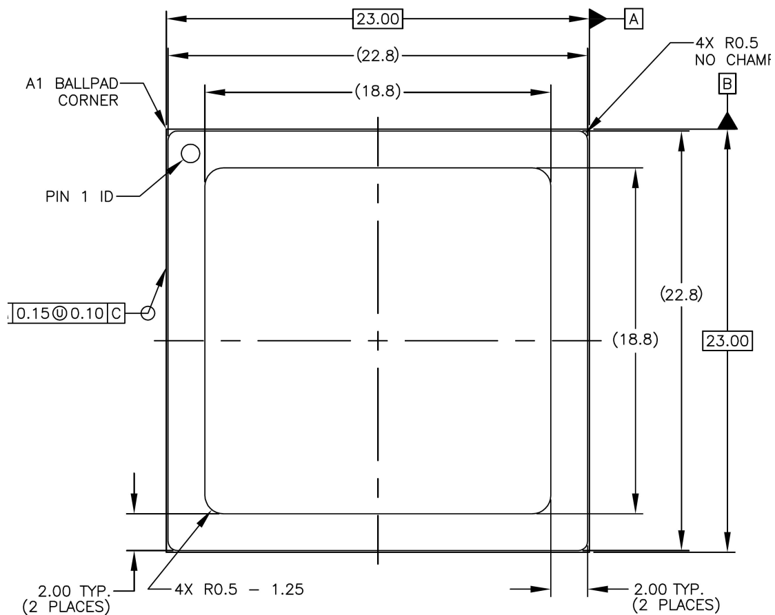
TOP VIEW
